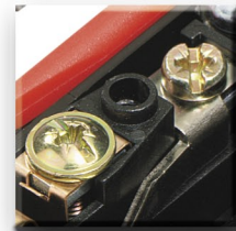
screw terminal for cables up to 2,5 mm 2
