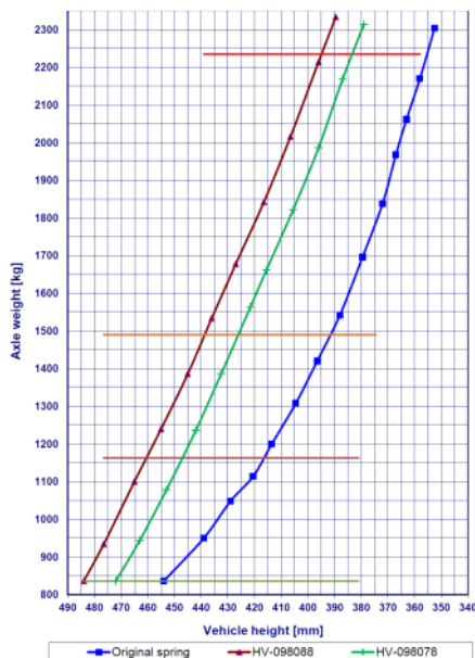
Rear axle characteristic
