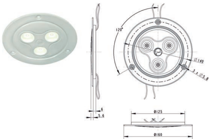
Einbau-Deckenleuchte IRIZIUM AR 600. Aluminium weiß. Recessed ceiling light IRIZIUM AR 600. White aluminium.
