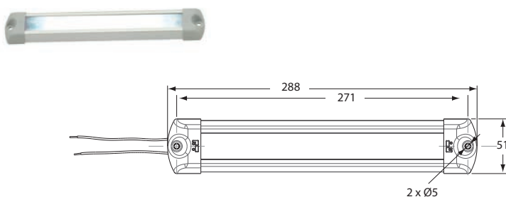
Beleuchtungsleiste, Aluminium, LEDs. Aluminium leds strip light.
