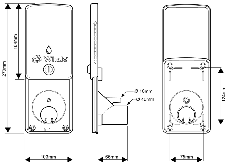
Figure 5. Onboard Tank Fill Socket Dimensional Drawings
