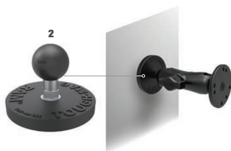
2 6 MAGNETS Max. weight 11lb 66mm diameter base
