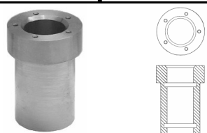
Weld-In Adapter For Fuel or Hydraulic Tanks
