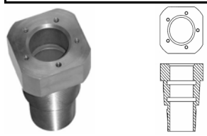
Threaded Adapter Fits 1-1/2" & 2" NPT Couplings
