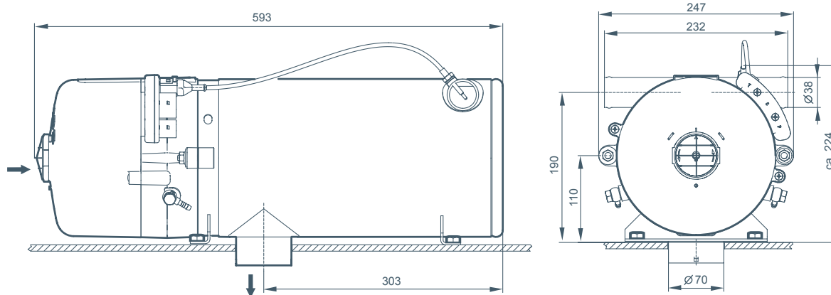
Thermo E installation dimensions
