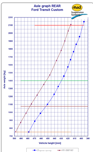
Power Spring Characteristic HV-068160
