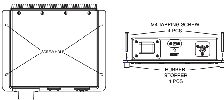
TUNER MOUNTING
