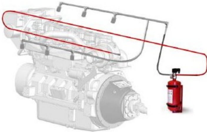
Cylinder with the valve 10 Systems C (EA,FA,NO)10
